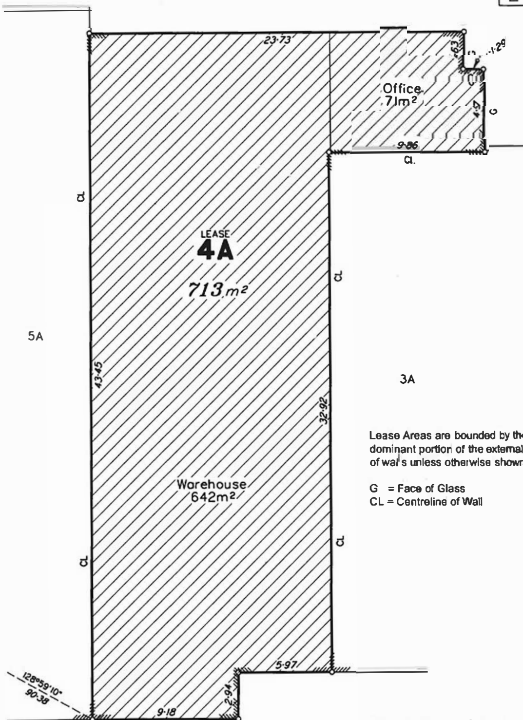
DIAGRAM A GROUND FLOOR SCALE 1:200
